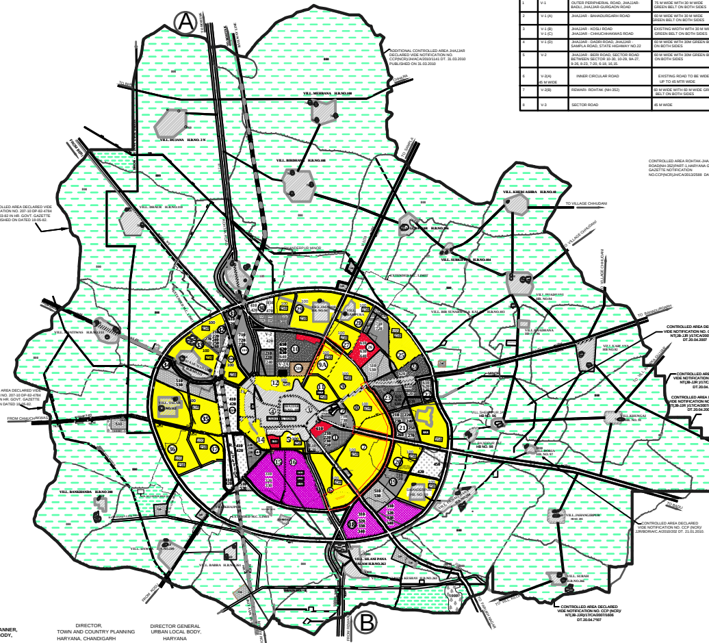
LAND RESERVATION FOR MAJOR ROADS
